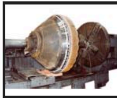
CRUSHER REPAIR
